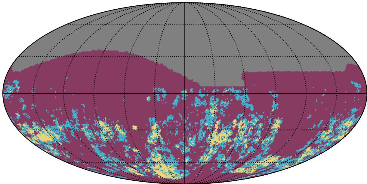
noroll_v3.4_10yrs z band: Gaps_7hr
