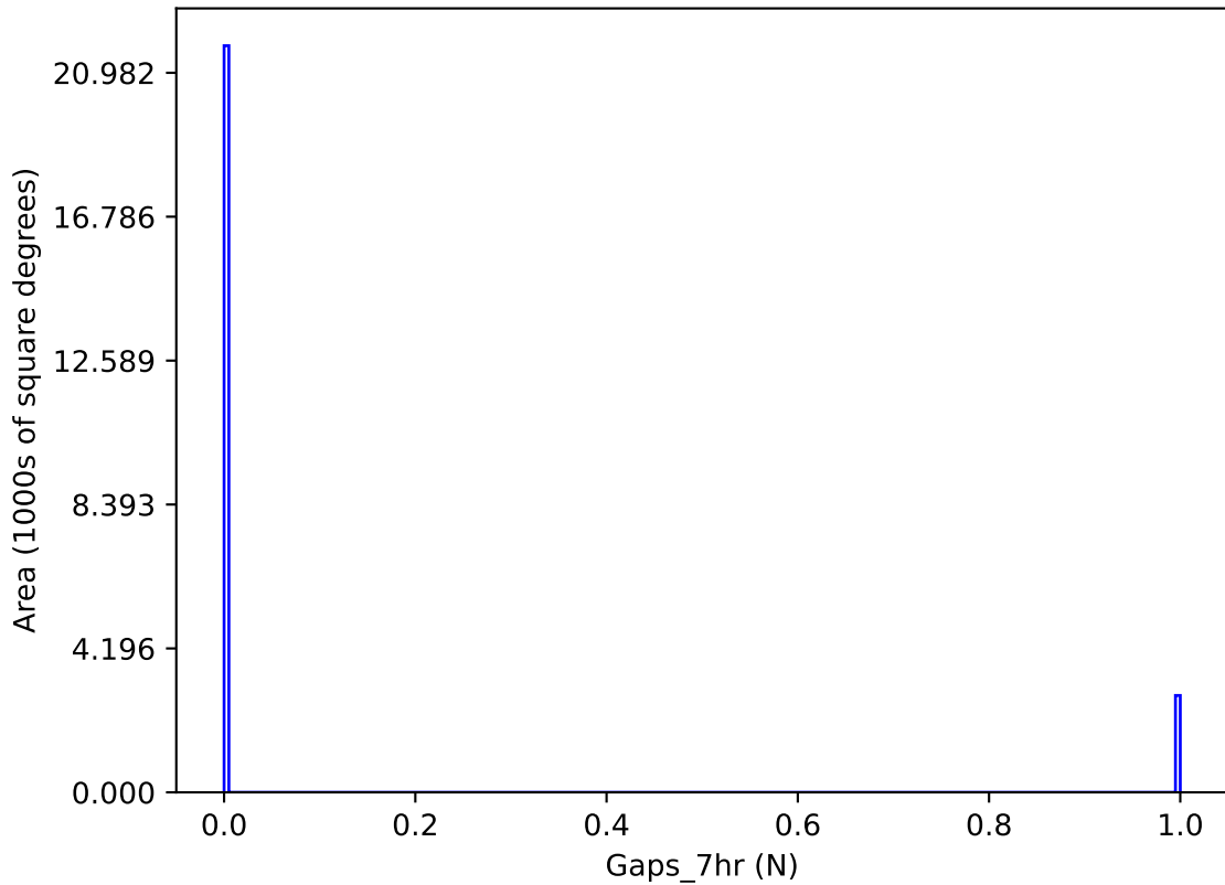
noroll_v3.4_10yrs y band: Gaps_7hr
