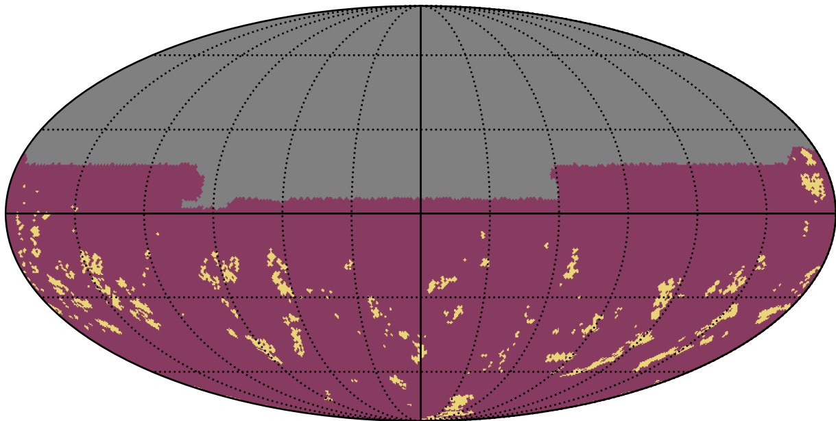
noroll_v3.4_10yrs u band: Gaps_7hr
