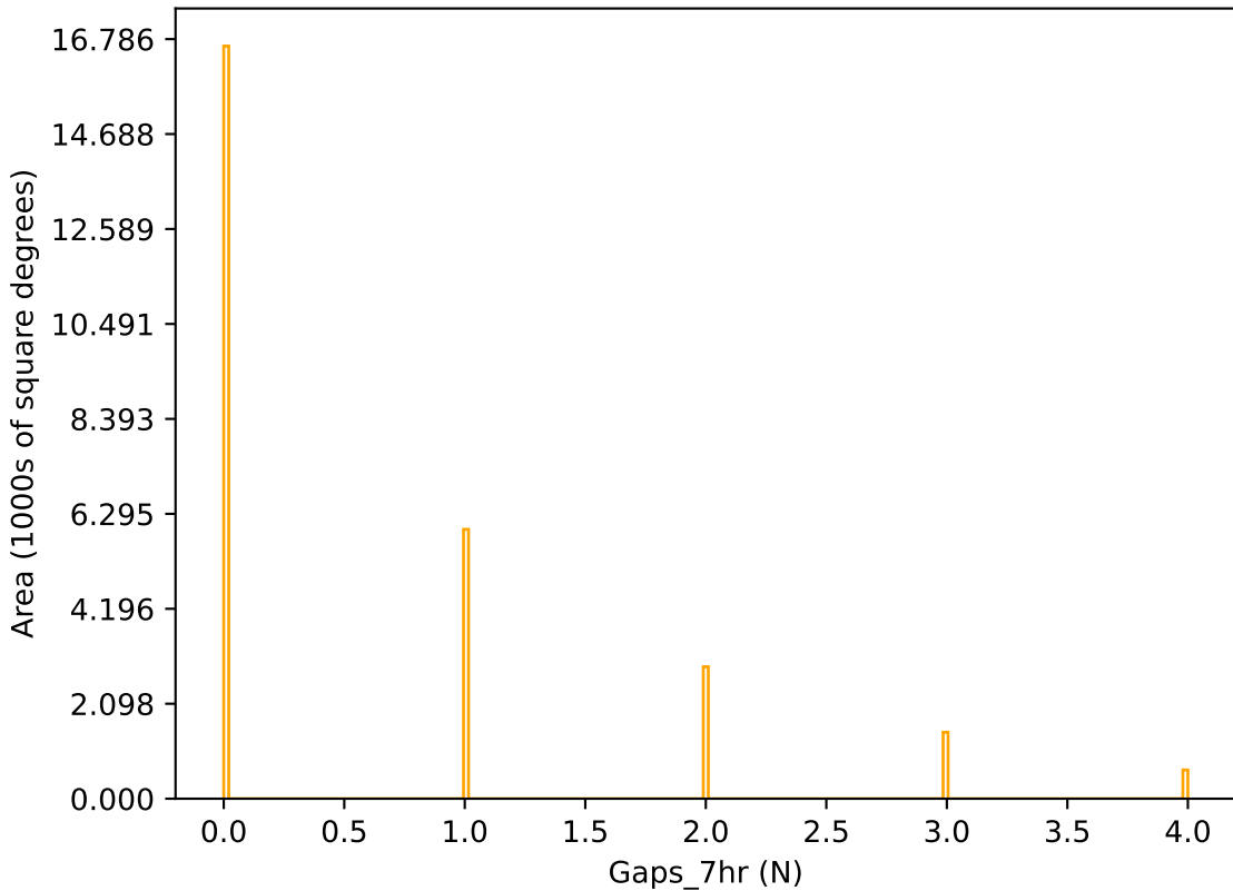
noroll_v3.4_10yrs r band: Gaps_7hr
