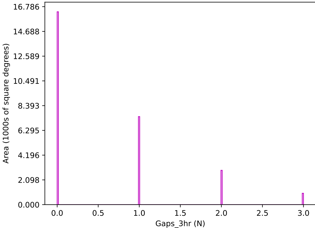
noroll_v3.4_10yrs z band: Gaps_3hr
