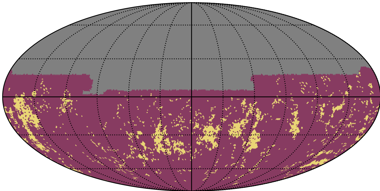
noroll_v3.4_10yrs u band: Gaps_3hr
