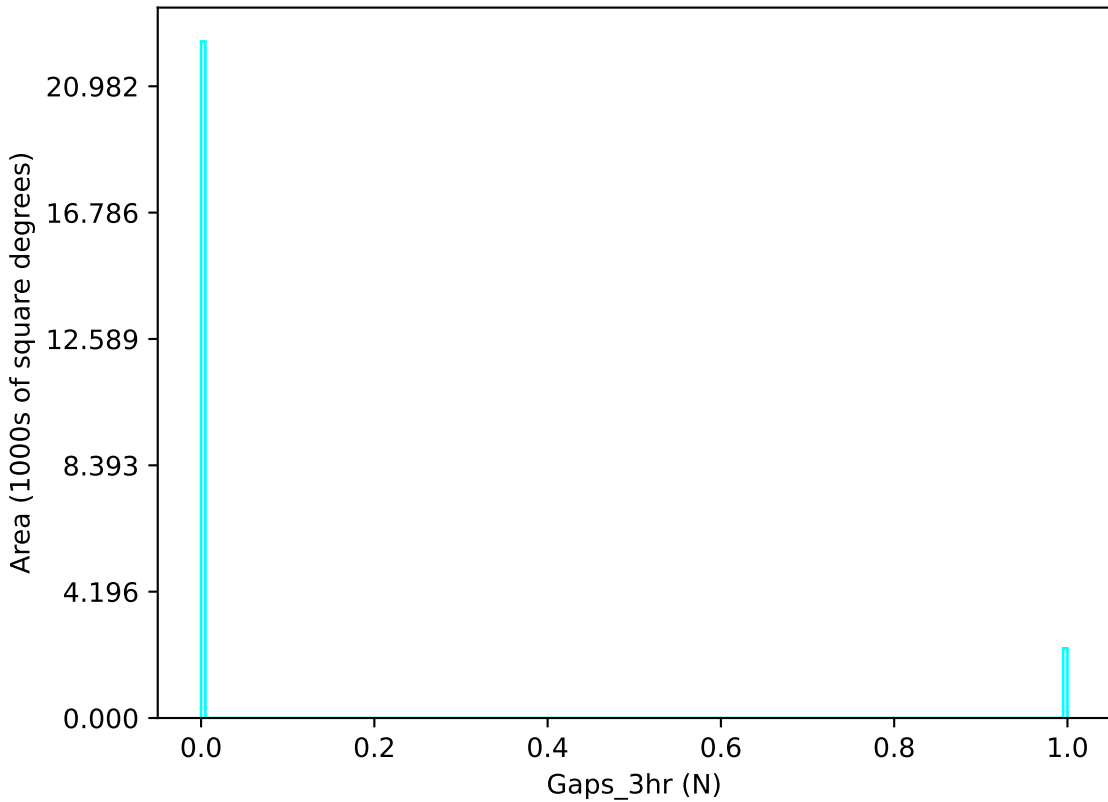
noroll_v3.4_10yrs u band: Gaps_3hr
