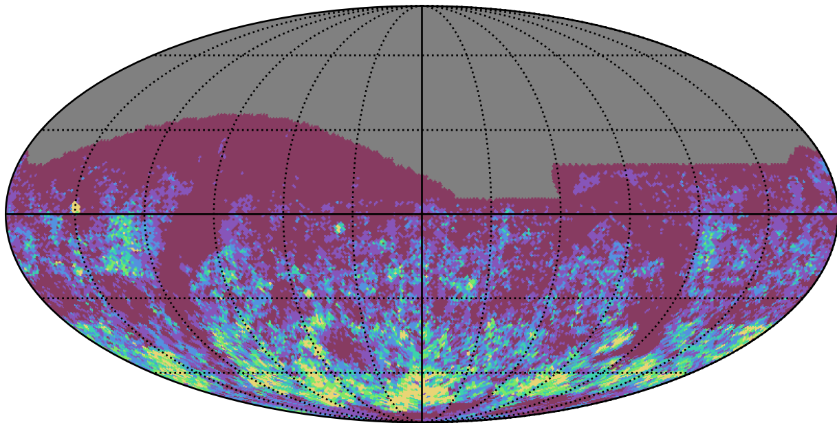
noroll_v3.4_10yrs r band: Gaps_3hr
