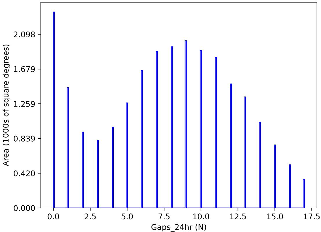
noroll_v3.4_10yrs y band: Gaps_24hr
