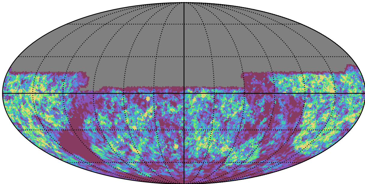
noroll_v3.4_10yrs u band: Gaps_24hr
