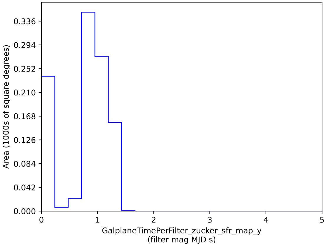
noroll_v3.4_10yrs : GalplaneTimePerFilter_zucker_sfr_map_y
