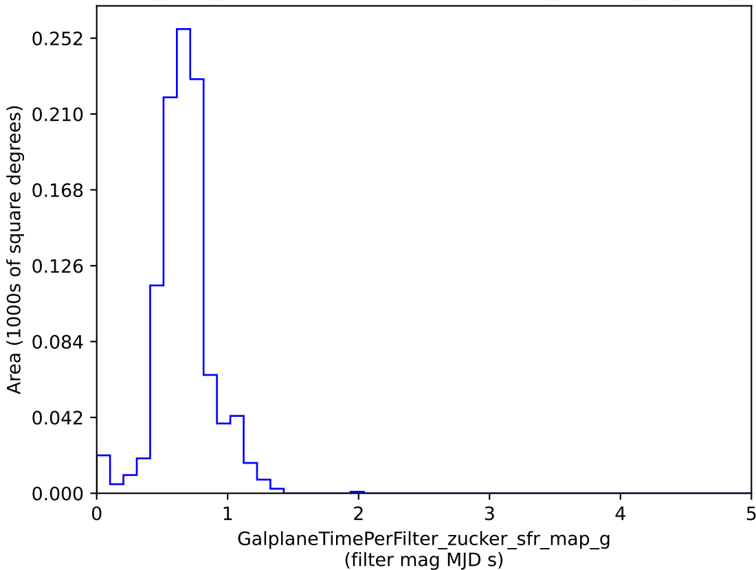
noroll_v3.4_10yrs : GalplaneTimePerFilter_zucker_sfr_map_g
