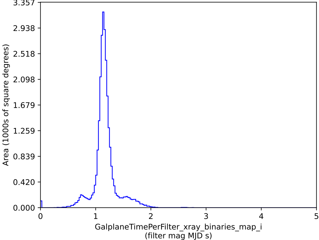
noroll_v3.4_10yrs : GalplaneTimePerFilter_xray_binaries_map_i
