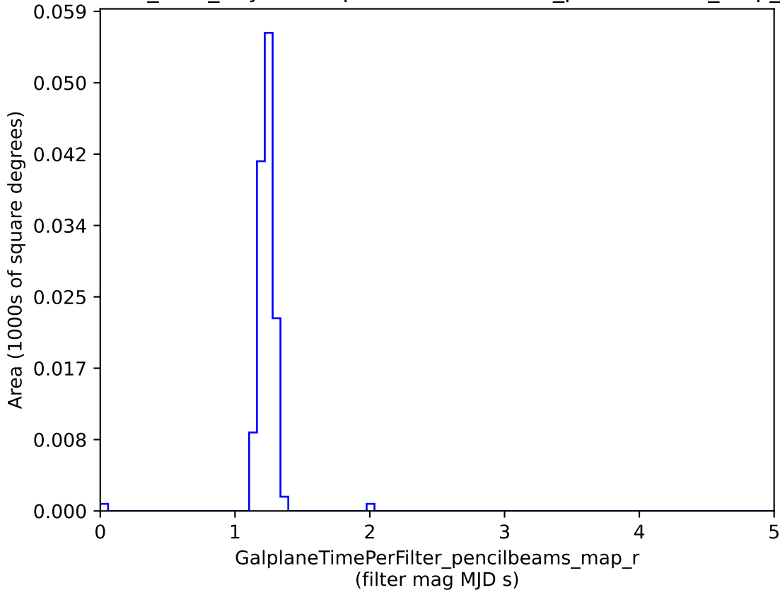
noroll_v3.4_10yrs : GalplaneTimePerFilter_pencilbeams_map_r
