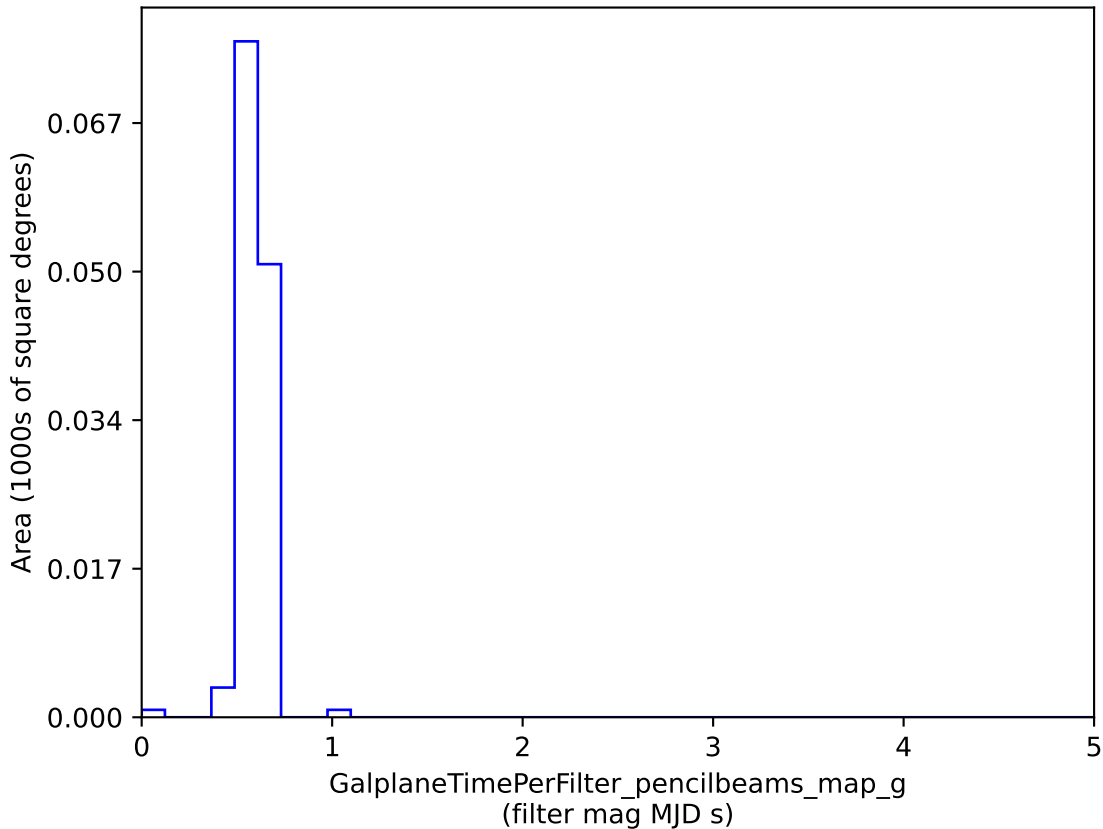
noroll_v3.4_10yrs : GalplaneTimePerFilter_pencilbeams_map_g
