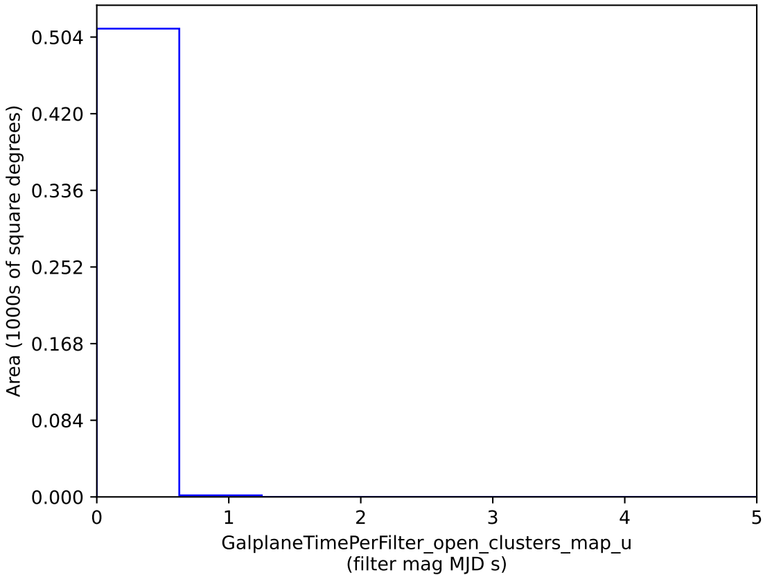
noroll_v3.4_10yrs : GalplaneTimePerFilter_open_clusters_map_u
