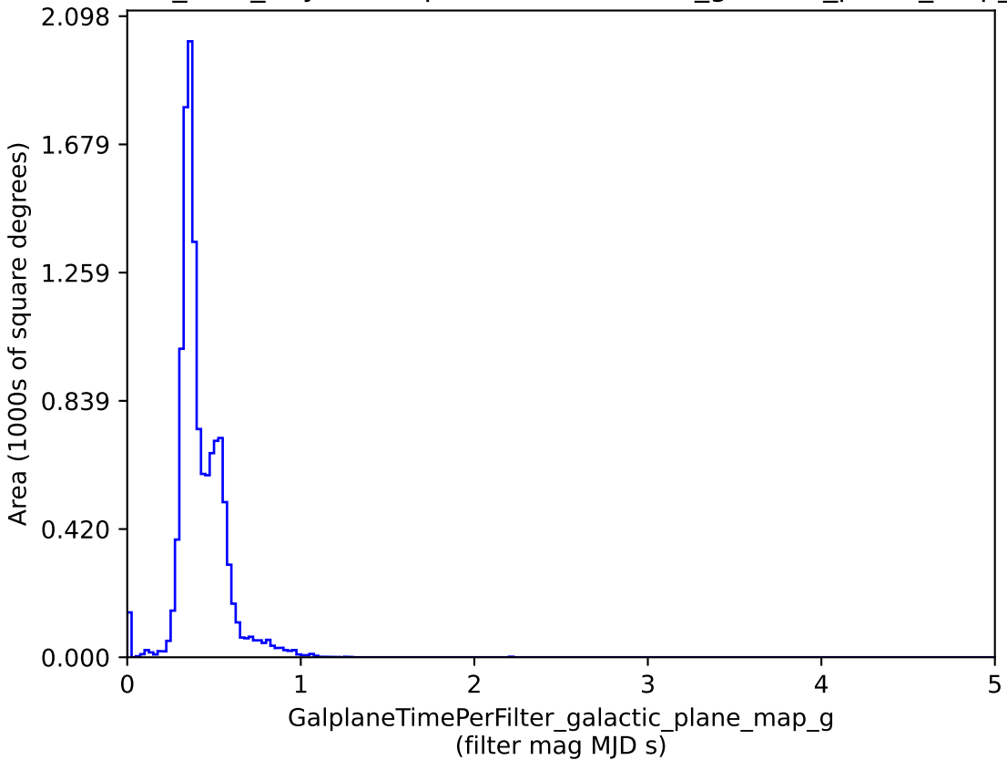
noroll_v3.4_10yrs : GalplaneTimePerFilter_galactic_plane_map_g
