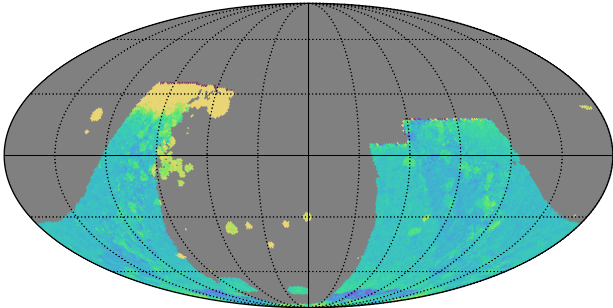
noroll_v3.4_10yrs : GalplaneTimePerFilter_combined_map_z
