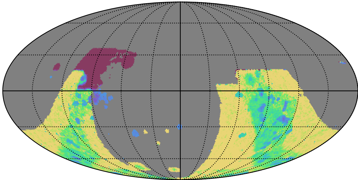
noroll_v3.4_10yrs : GalplaneTimePerFilter_combined_map_y
