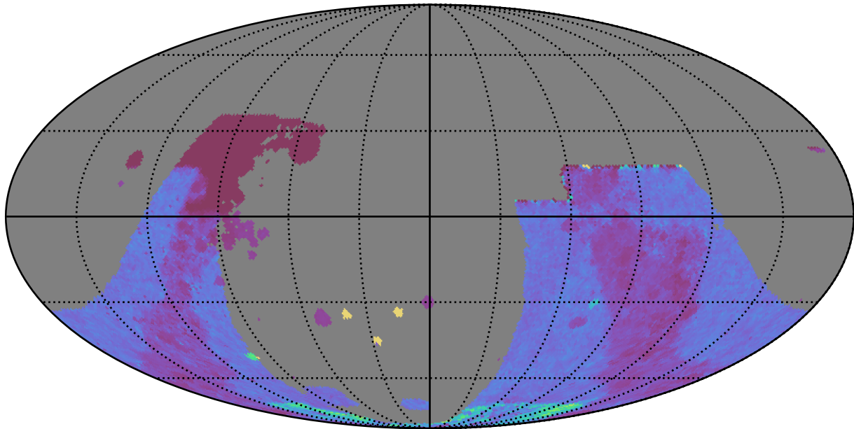
noroll_v3.4_10yrs : GalplaneTimePerFilter_combined_map_u
