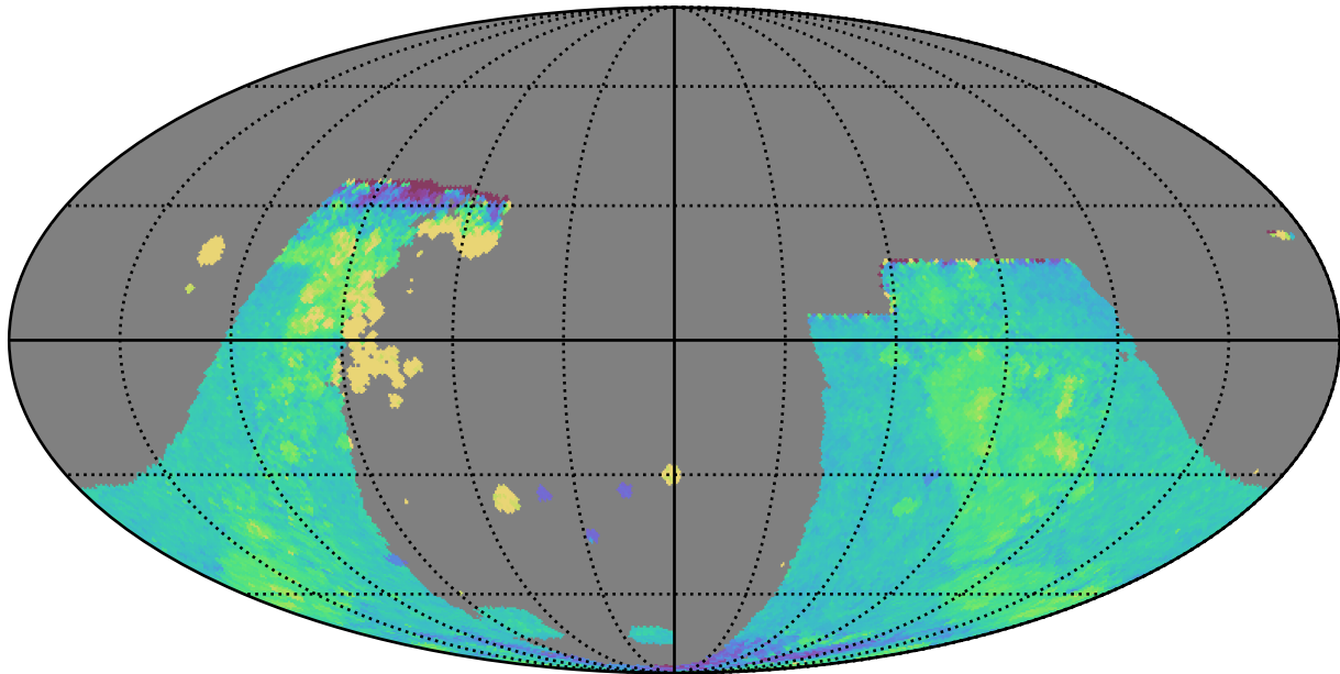
noroll_v3.4_10yrs : GalplaneTimePerFilter_combined_map_r
