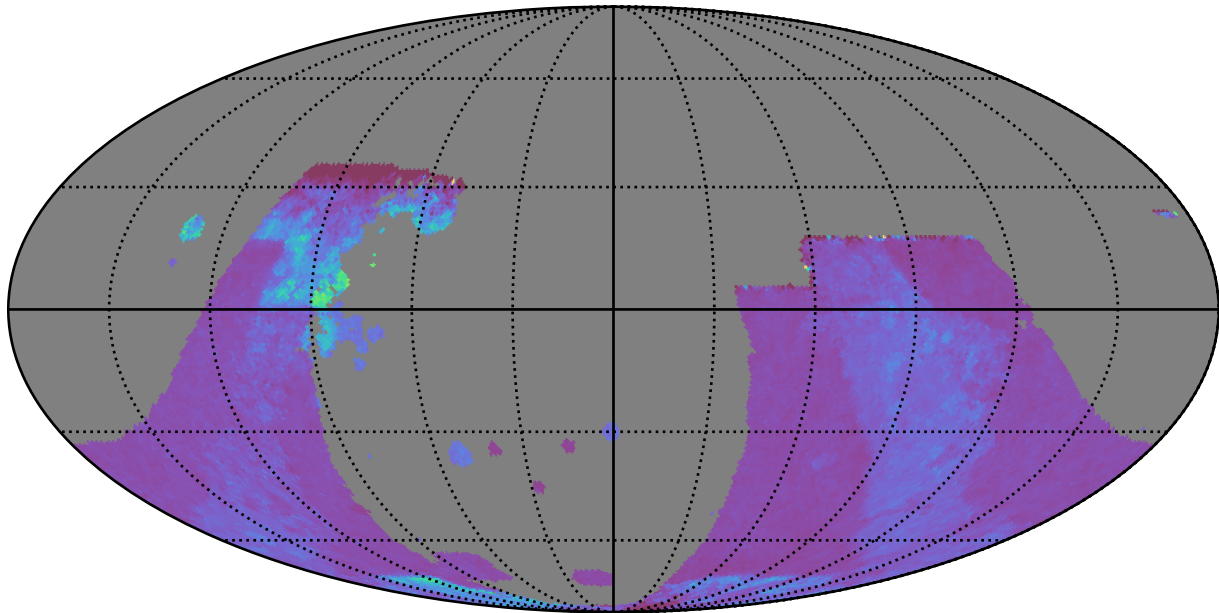
noroll_v3.4_10yrs : GalplaneTimePerFilter_combined_map_g
