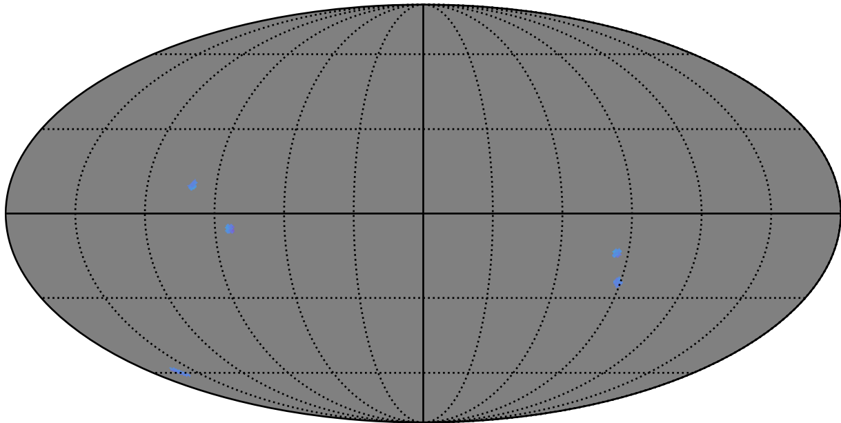
noroll_v3.4_10yrs : GalplaneTimePerFilter_bonito_sfr_map_g
