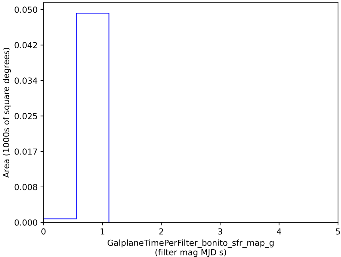
noroll_v3.4_10yrs : GalplaneTimePerFilter_bonito_sfr_map_g
