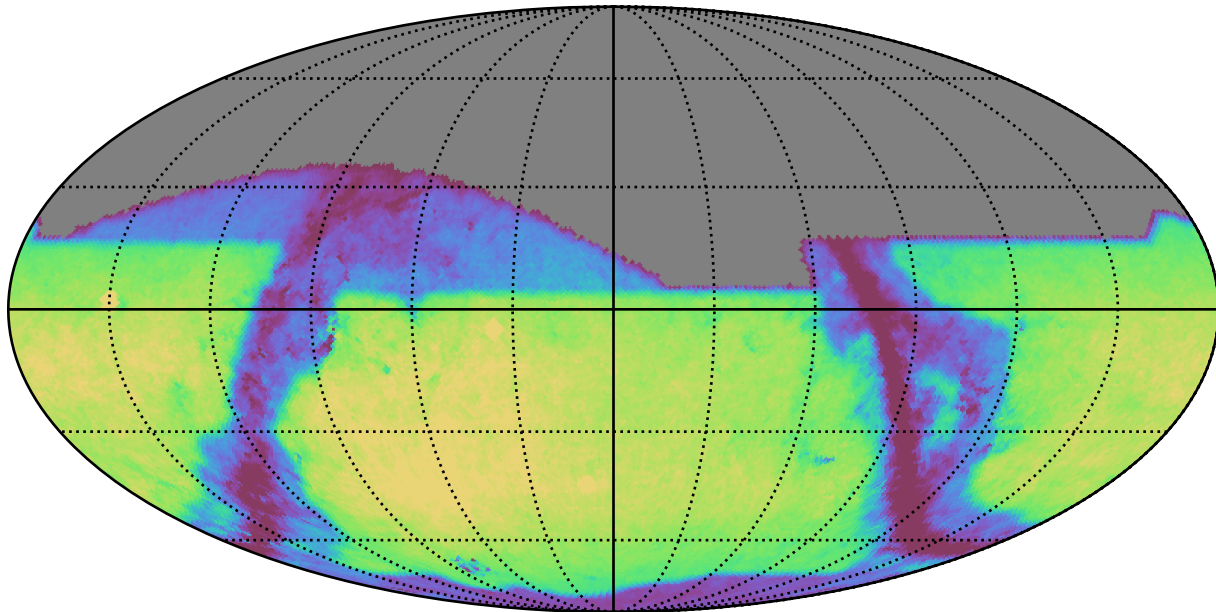
noroll_v3.4_10yrs z: GalaxyCountsMetricExtended
