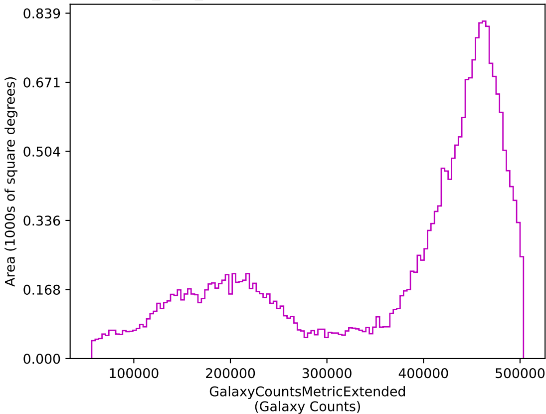
noroll_v3.4_10yrs z: GalaxyCountsMetricExtended
