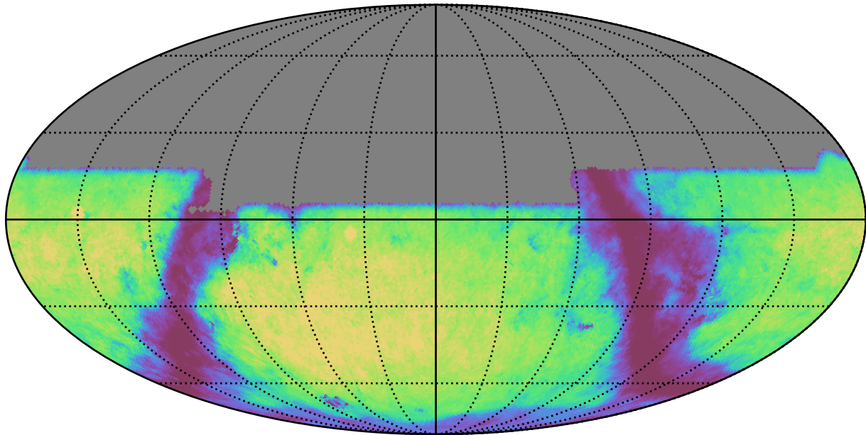
noroll_v3.4_10yrs u: GalaxyCountsMetricExtended
