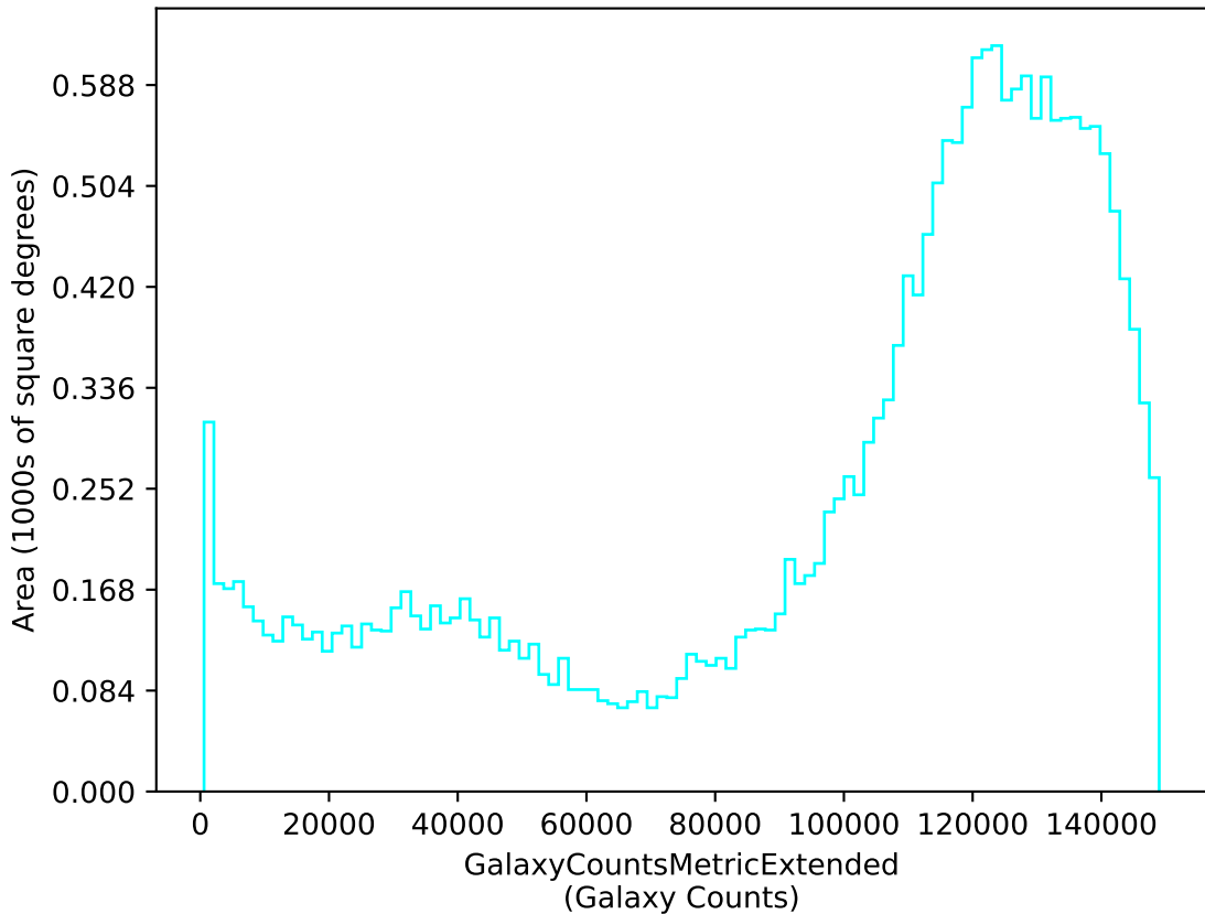
noroll_v3.4_10yrs u: GalaxyCountsMetricExtended
