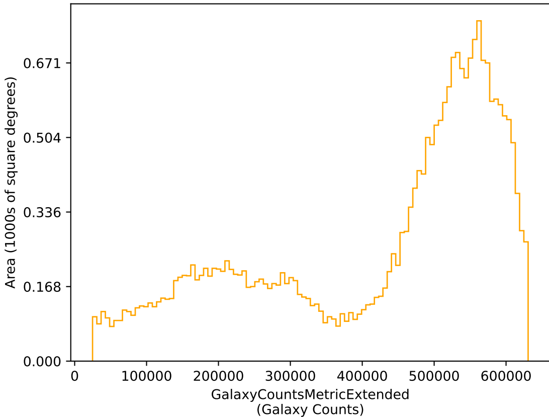
noroll_v3.4_10yrs r: GalaxyCountsMetricExtended
