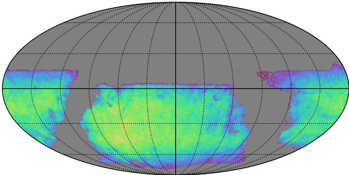
noroll_v3.4_10yrs i band non-DD year 9: ExgalM5WithCuts
