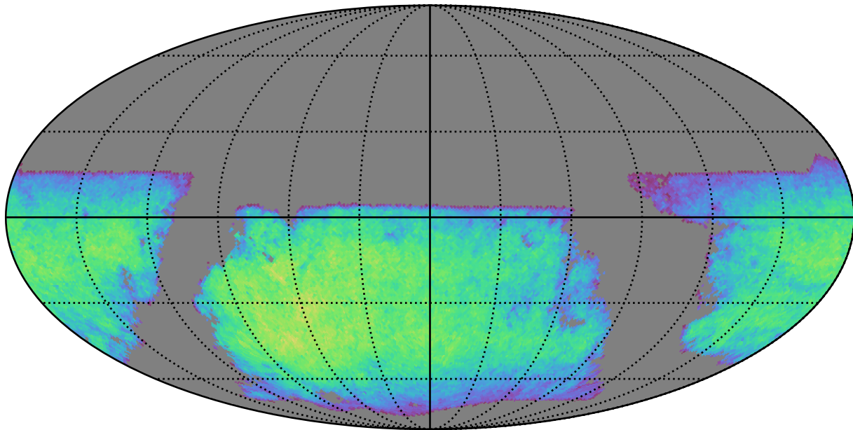
noroll_v3.4_10yrs i band non-DD year 6: ExgalM5WithCuts
