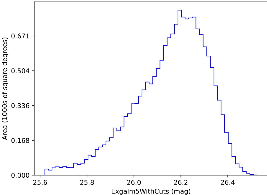
noroll_v3.4_10yrs i band non-DD year 6: ExgalM5WithCuts
