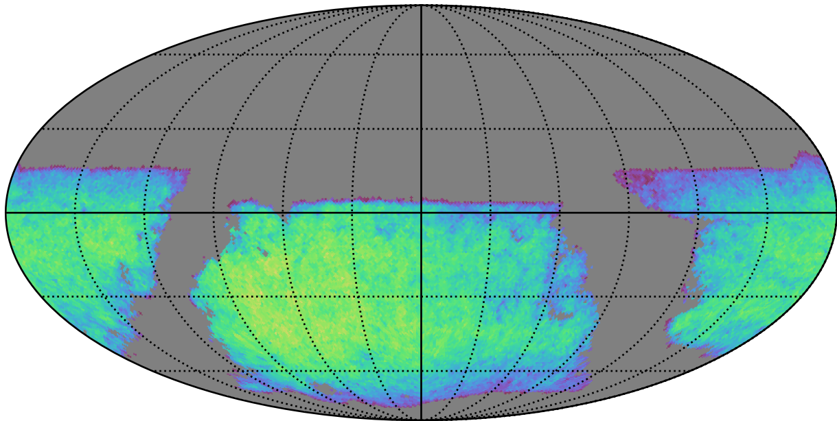
noroll_v3.4_10yrs i band non-DD year 3: ExgalM5WithCuts
