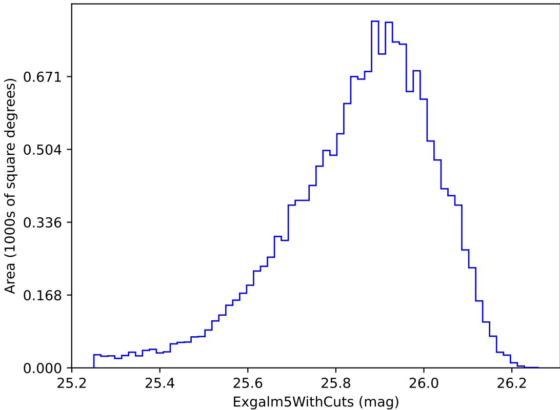
noroll_v3.4_10yrs i band non-DD year 3: ExgalM5WithCuts
