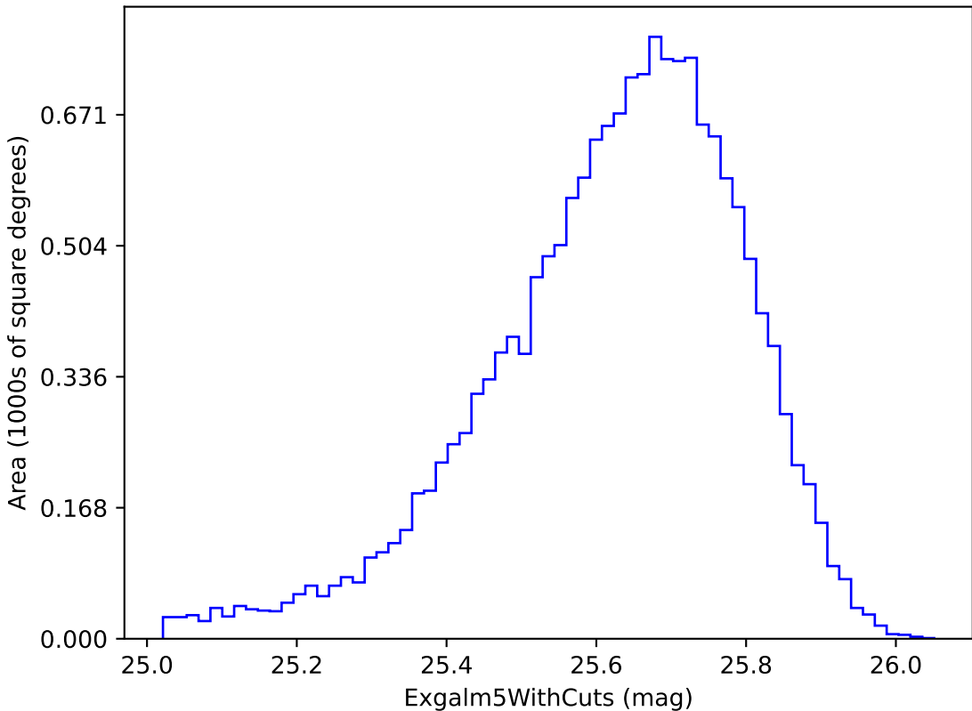
noroll_v3.4_10yrs i band non-DD year 2: ExgalM5WithCuts
