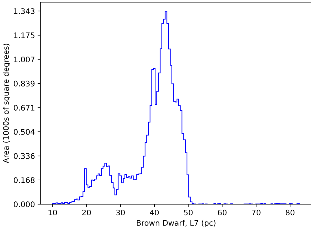
noroll_v3.4_10yrs : Brown Dwarf, L7
