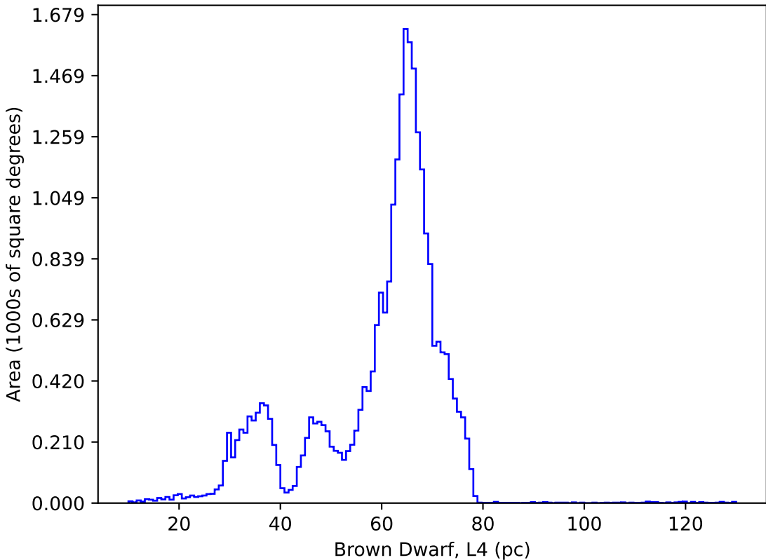
noroll_v3.4_10yrs : Brown Dwarf, L4
