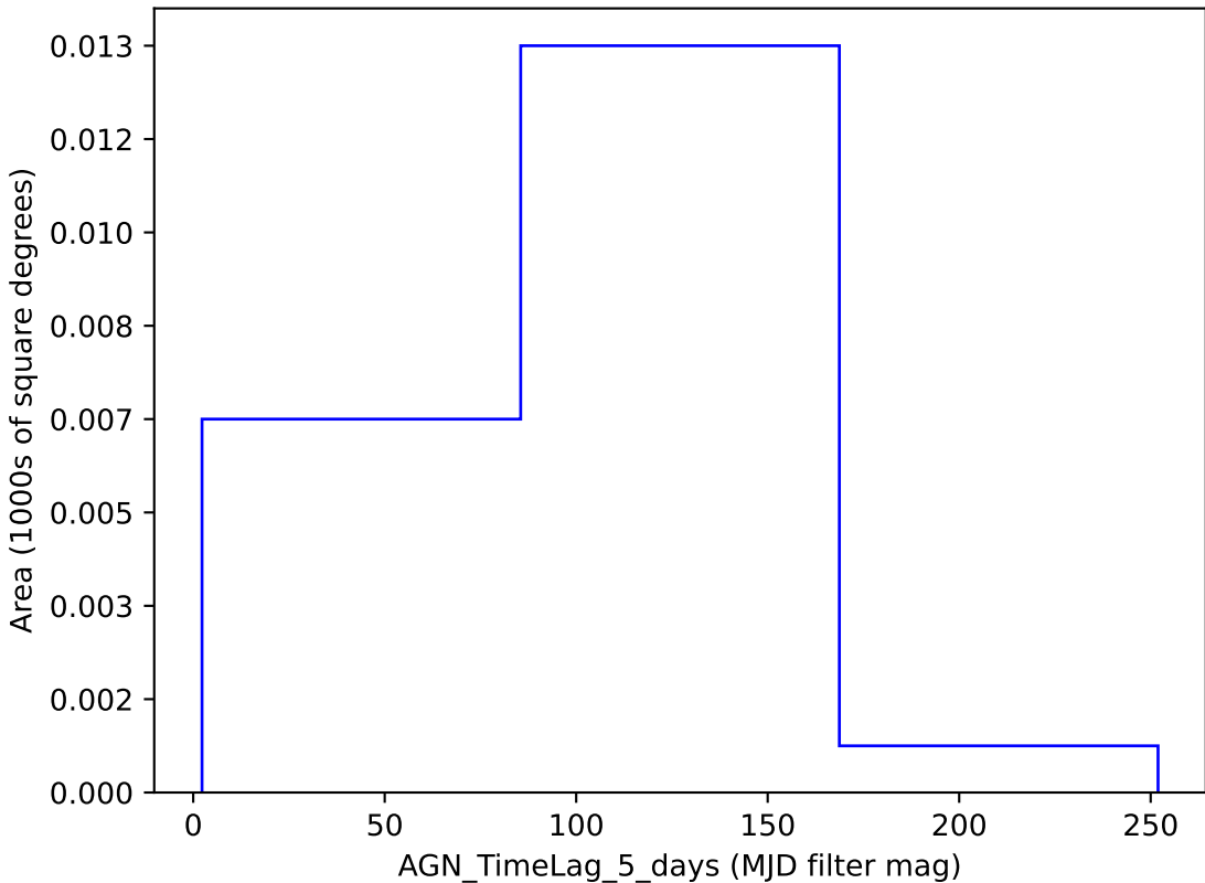
noroll_v3.4_10yrs y band: AGN_TimeLag_5_days
