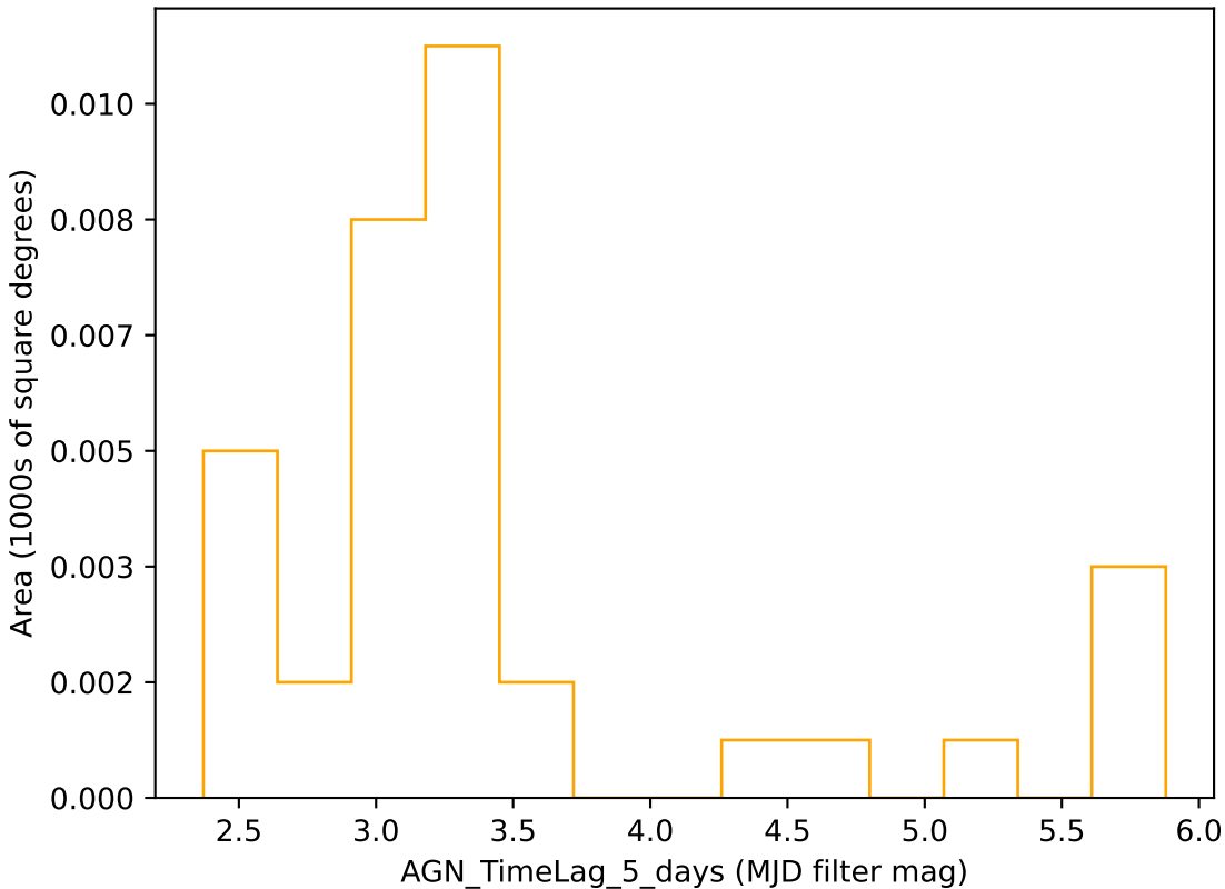
noroll_v3.4_10yrs r band: AGN_TimeLag_5_days
