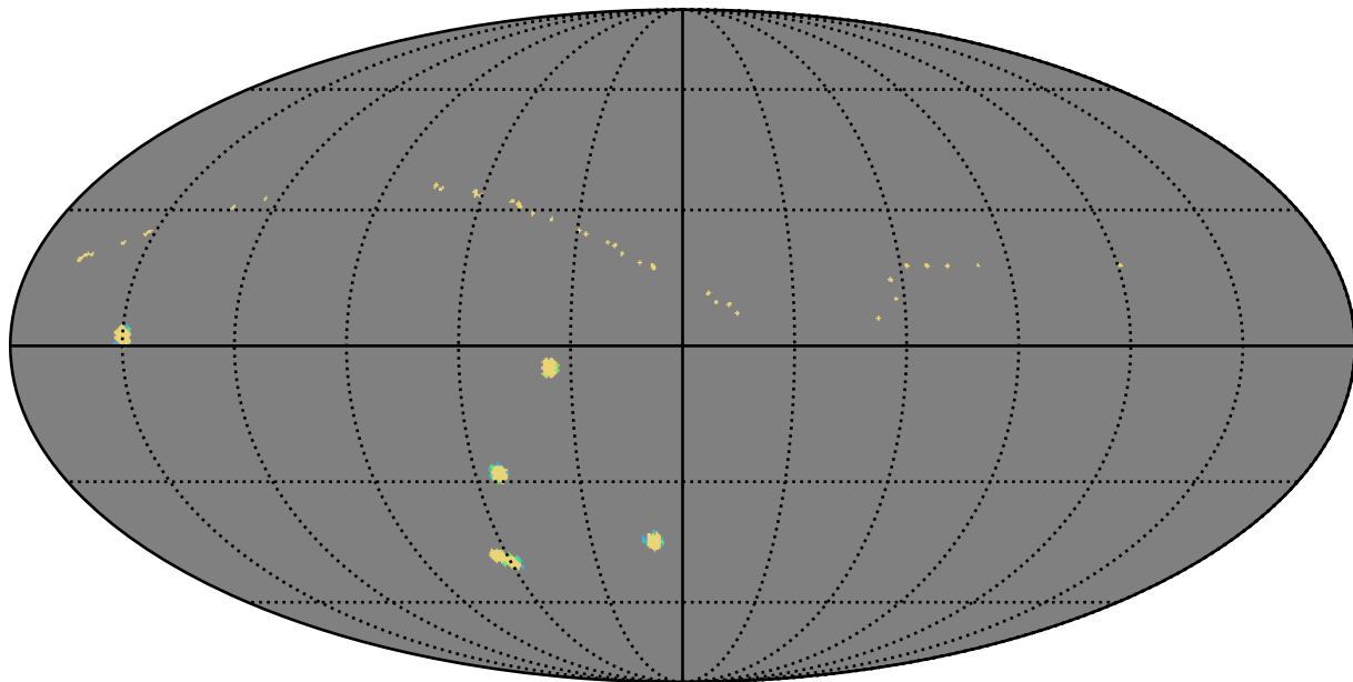
noroll_v3.4_10yrs all bands: AGN_TimeLag_5_days
