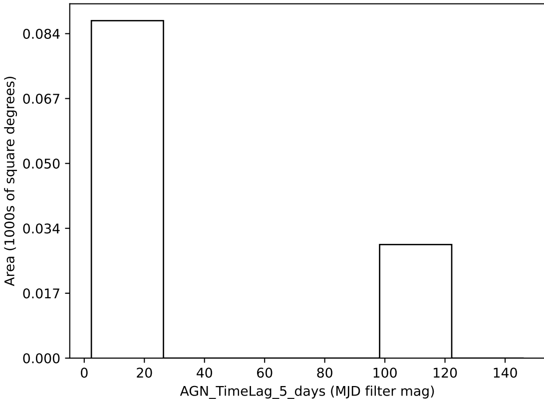
noroll_v3.4_10yrs all bands: AGN_TimeLag_5_days
