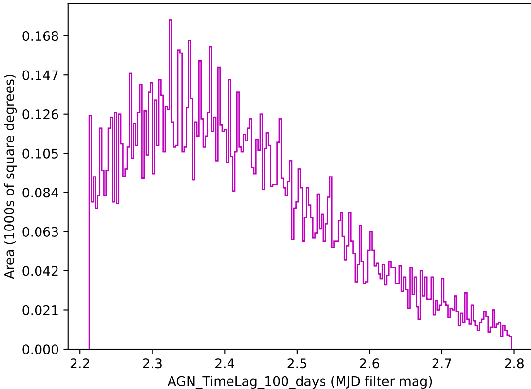
noroll_v3.4_10yrs z band: AGN_TimeLag_100_days
