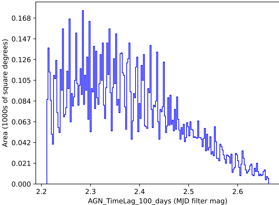
noroll_v3.4_10yrs y band: AGN_TimeLag_100_days
