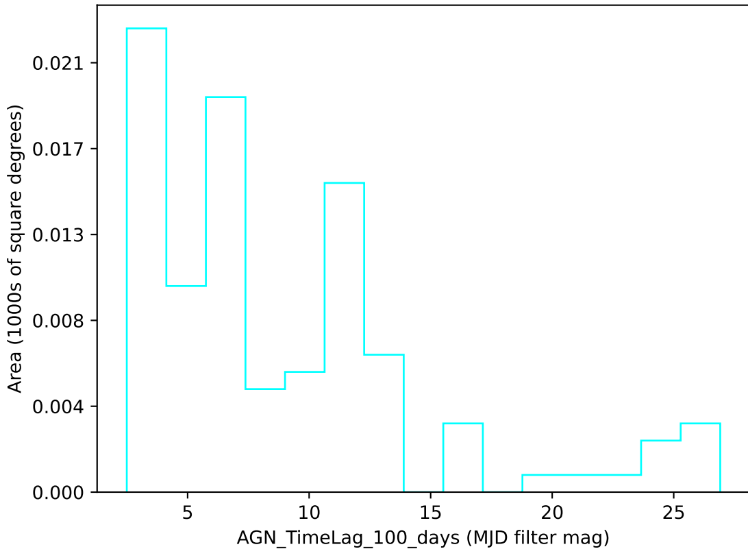
noroll_v3.4_10yrs u band: AGN_TimeLag_100_days
