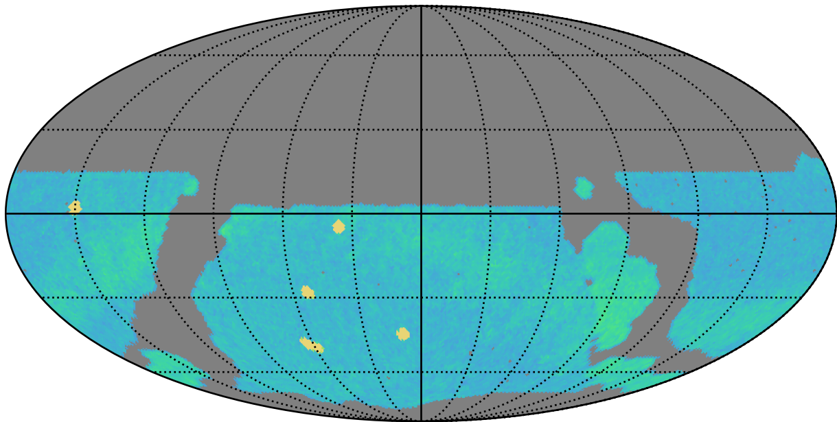
noroll_v3.4_10yrs r band: AGN_TimeLag_100_days
