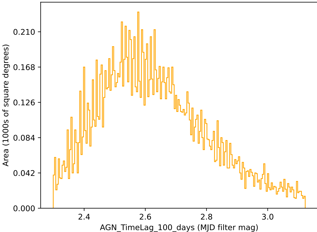
noroll_v3.4_10yrs r band: AGN_TimeLag_100_days
