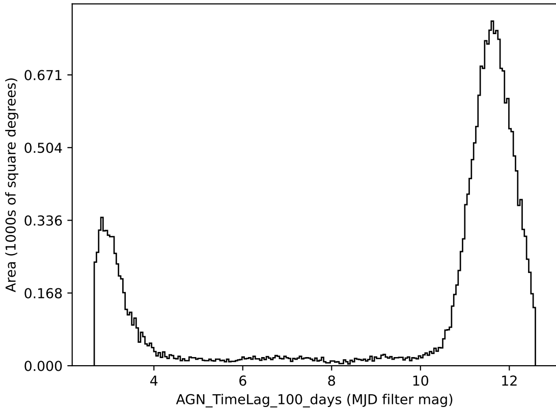
noroll_v3.4_10yrs all bands: AGN_TimeLag_100_days
