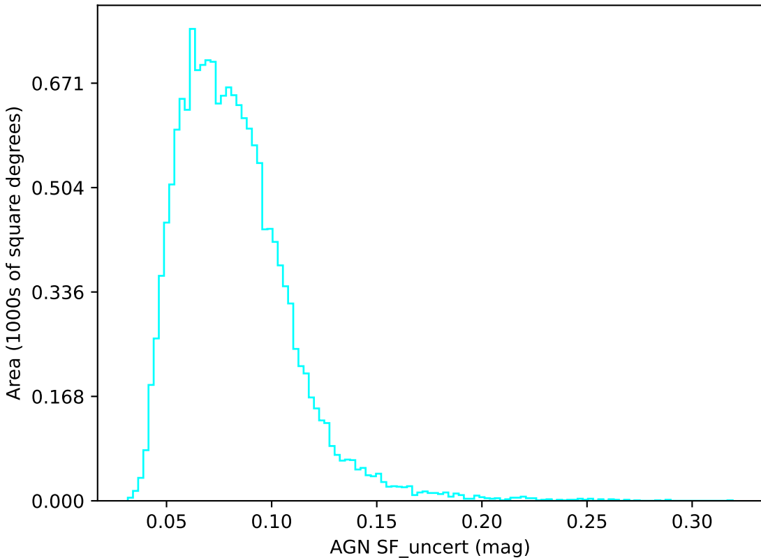
noroll_v3.4_10yrs u band: AGN SF_uncert
