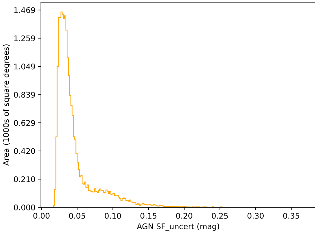
noroll_v3.4_10yrs r band: AGN SF_uncert
