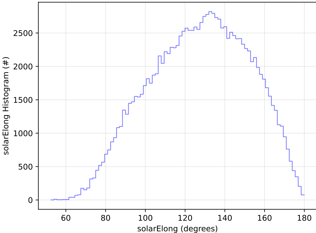
noroll_v3.4_10yrs WFD u band: solarElong Histogram
